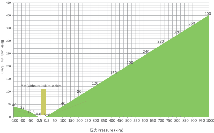
FFM-110-1*压力-漏率范围(表1) Pressure-Leak rate Range (table 1)
